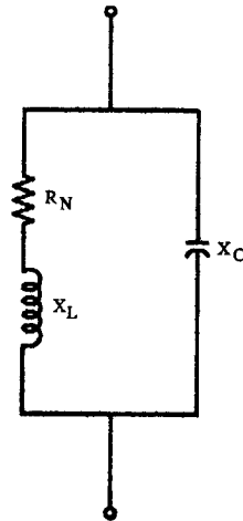
Fig. 10. Neutral R-L-C impedance.
