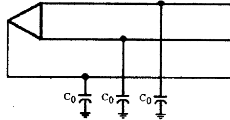
Fig. 3. Capacitive grounding.
