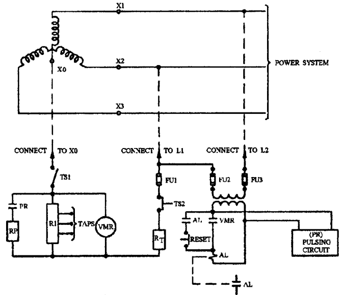
Fig. 8. High-resistance grounded system detail schematic. AL: alarm/tripping relay. R1: tapped grounding resistor. RP: pulsing resistor. PR: pulsing relay. TS1: resistor disconnect switch. TS2: ground test switch. VMR: voltage meter relay. FU1, FU2, FU3: fuses.
