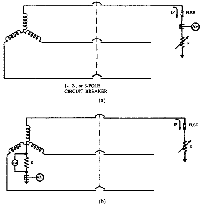
Fig. 12. (a) Test circuit for measuring capacitive current. (b) Test circuit for measuring voltage and current at grounding resistor.
