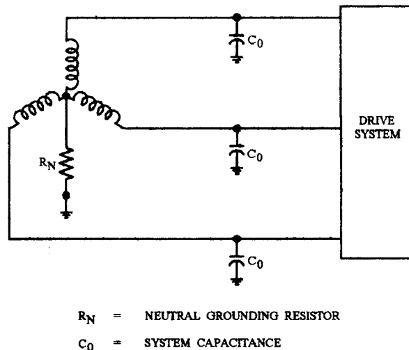
Fig. 9. High-resistance neutral grounding with high-frequency filtering capacitor.
