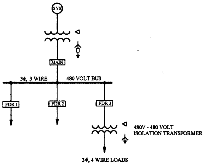
Fig. 5. High-resistance grounded main system with three-phase four-wire lighting loads.
